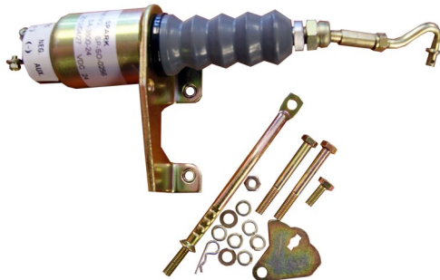
12V 2 FIS RSV BOSCH KIT MODEL: 1751-12V / WOODWARD: SA-3800-12V
