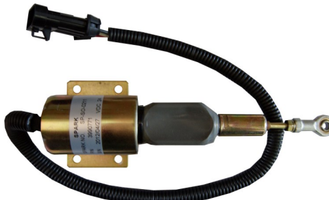
24V 3 FIS CUMMINS CUMMINS: 3990771 / WOODWARD: SA-4931-24V
