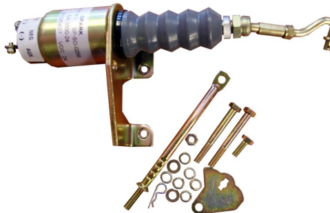
24V 2 FIS RSV BOSCH KIT MODEL: 1751-24V / WOODWARD: SA-3800-24V
